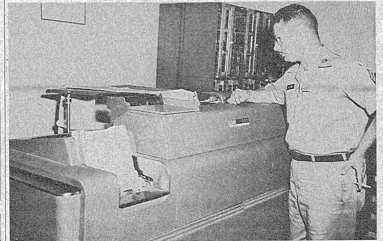
ACCOUNTING MACHINE - S/Sgt Elmo Newman, operates an IBM Accounting machine which prints the individual pay voucher from the data punched on the cards.
